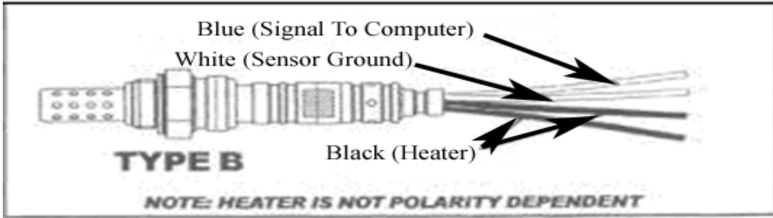
Figure 1 : Universal Oxygen Sensor Wiring for Type B Sensor
