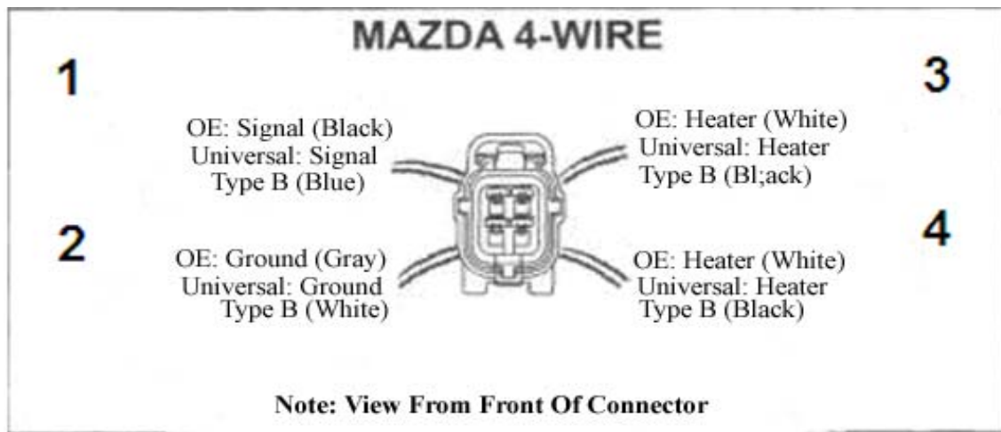
Figure 2: Mazda Miata 4-wire sensor wiring scheme.
